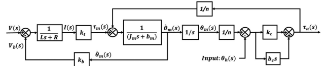
Fig. 6. Block diagram of human-exoskeleton open loop system.
